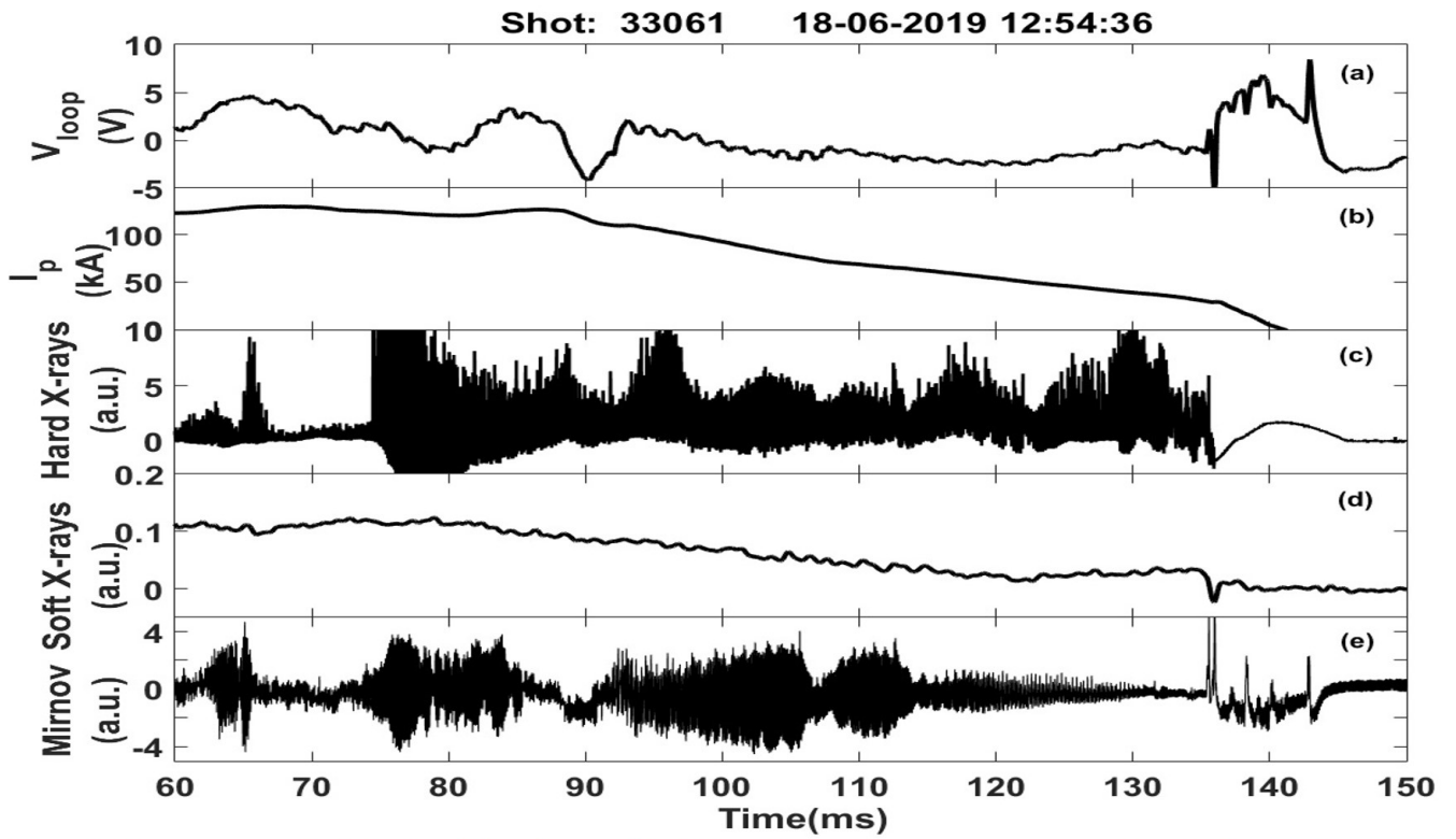
Fig. 3. Time traces of ADITYA-U discharge (#33061) shows plasma parameters for RE beam formation
